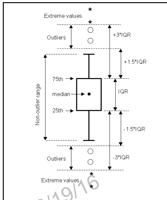
Figure A-1. Ranges of outliers and extremes in box-and-whisker plots (after Statsoft 1998). IQR is the interquartile range.
