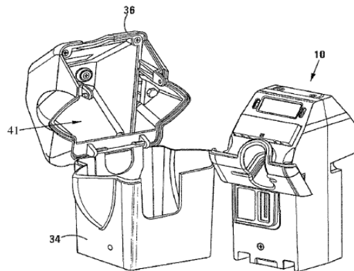
Figure 7 of the '054 patent shows the parking meter device alongside the empty housing, with the cover panel (36) again in the open position:
