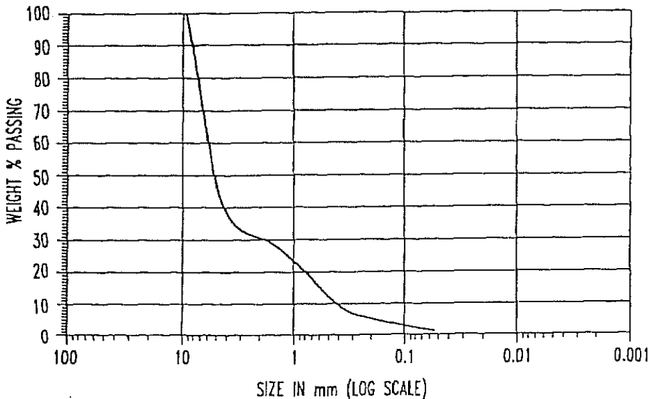
PARTICLE SIZE DISTRIBUTION CURVE
