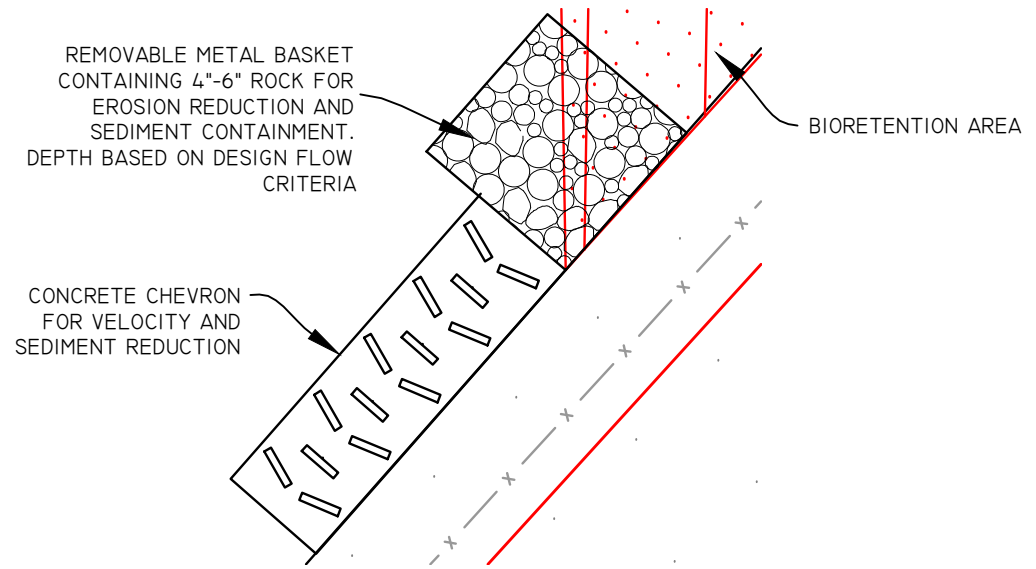
PRETREATMENT TYP. DETAIL
