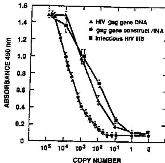
Figure 1. Quantification of infectious human immunodeficiency virus (HIV III ) RNA, HIV gag gene DNA, and cRNA gag gene construct copy number by polymerase chain reaction.
