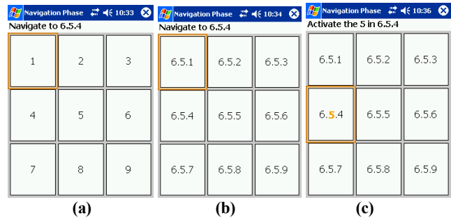
Figure 5. Example gesture study environment states: (a) the top level, (b) the third level after ACTIVATE is performed on 6.5, (c) highlighting within a cell.
