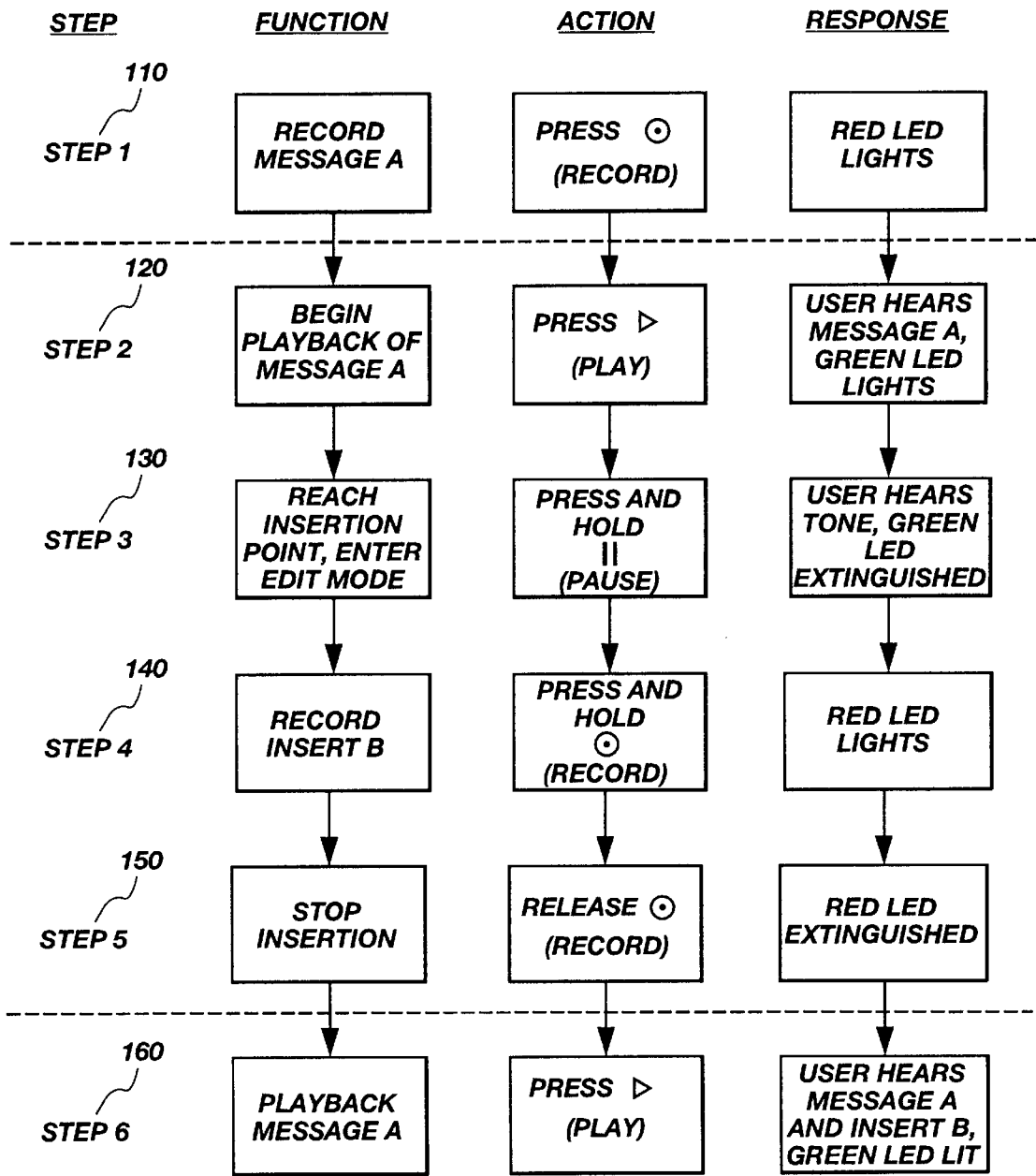
Fig. 2A: RANDOM INSERTION
