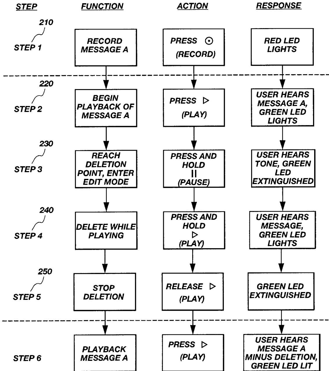
Fig. 3A: RANDOM DELETION
