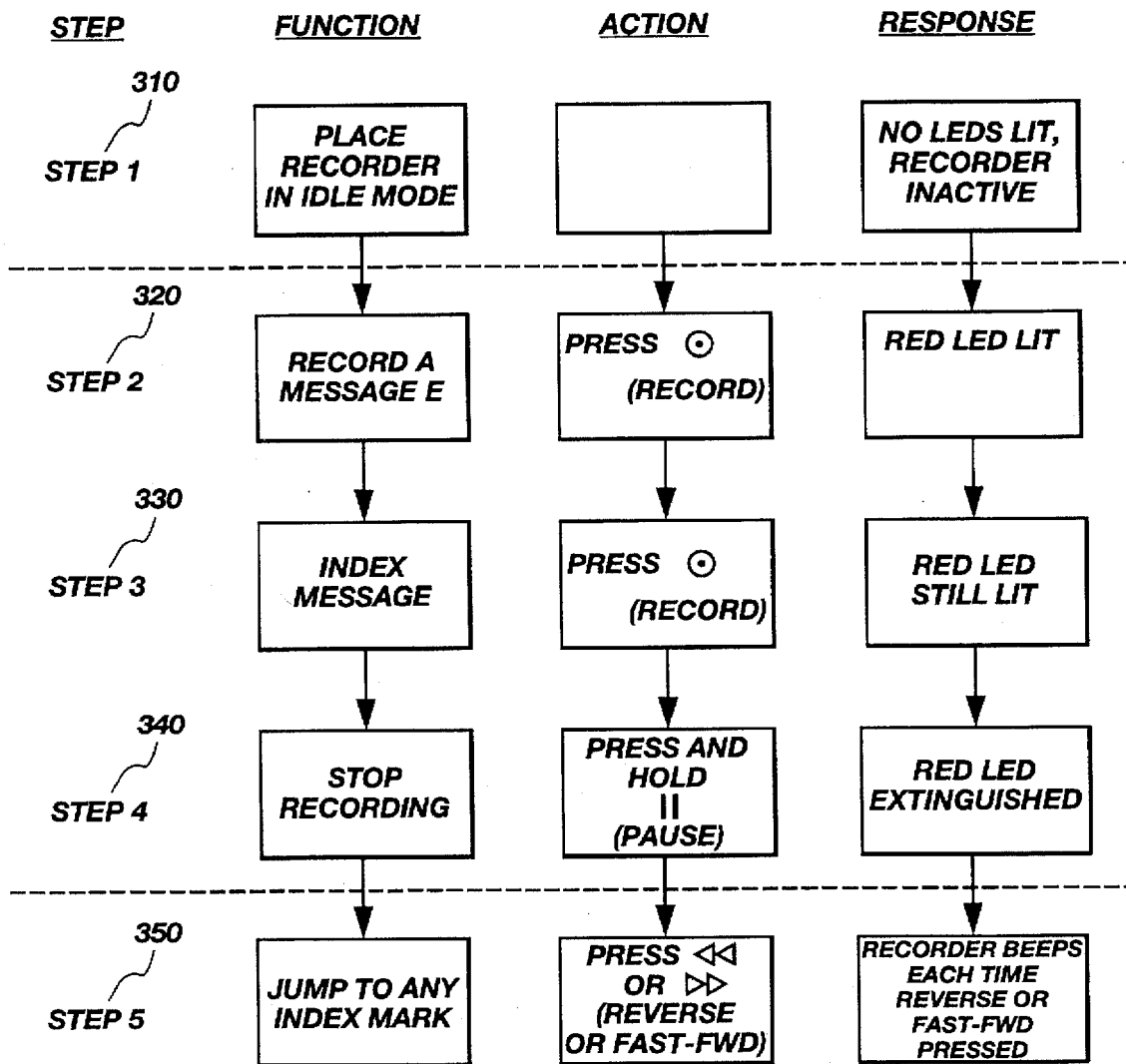
Fig. 4: INDEXING OF MESSAGE
