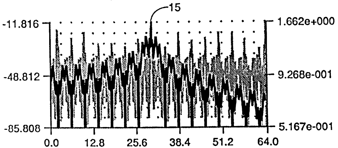
AMPLITUDE ON-OFF CARRIER MODULATION SPECTRUM
