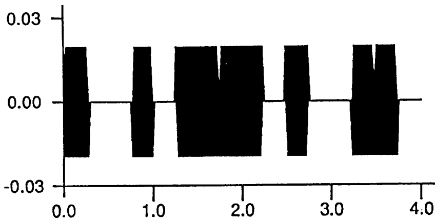
AMPLITUDE ON-OFF PLUS BIPHASE CARRIER MODULATION
