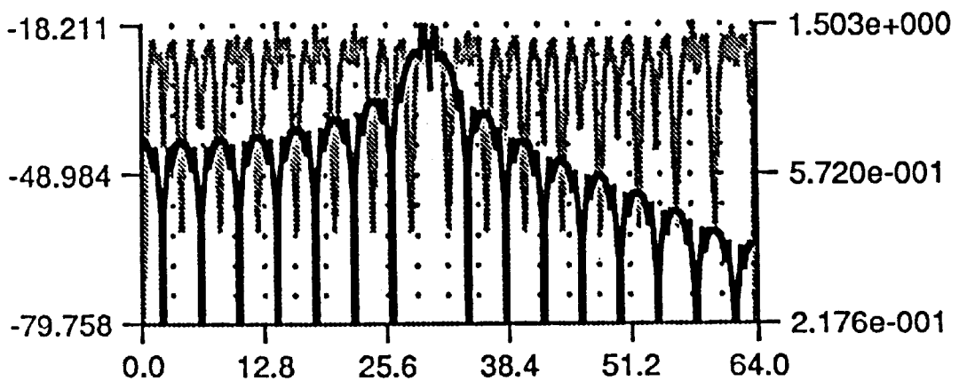
AMPLITUDE ON-OFF PLUS BIPHASE CARRIER MODULATION SPECTRUM
