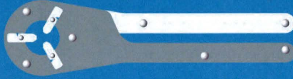
Close Status
