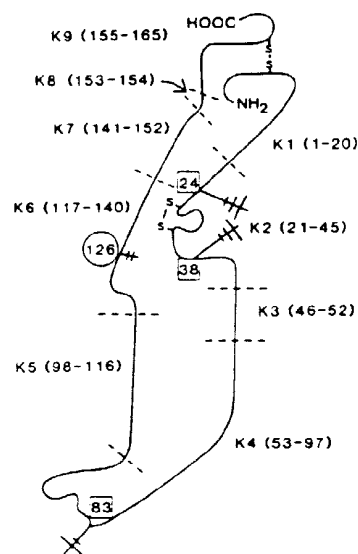
FIGURE 2: Predicted structure of human erythropoietin [adopted from references of McDonald et al. (1986) and Reçny et al. (1987)]. K1-K9 are peptides generated by Endo Lys-C, and the amino acid residue numbers are indicated in parentheses. The amino acid residues 24, 38, and 83 attach N-linked saccharides, whereas residue 126 attaches O-linked saccharides.
