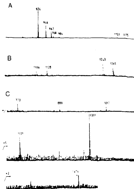
FIGURE 7: Fast atom bombardment mass spectra of peptides obtained from 0-126 (K6), N-24, and N-38 glycopeptides. The positive spectra were obtained on carbohydrate-free peptides. (A) Fractions 54-56, peptide D in Figure 4 (tryptic peptide from K6). The prominent ions at m/z 924, 946, and 962 correspond to [M + H]^+ , [M + Na]^+ , and [M + K]^+ for TITADTFR. Minor signals at m/z 1153 and 1175 could correspond to residues 41-50 or 125-143. (B) Fractions 47-52 in Figure 8A (N-24). The prominent ions at m/z 1243 and 1265 correspond to the molecular ion and its Na adduct for EAEDITG-(EtPy)-CAE. The ions at m/z 1106 and 1128 are probably due to a contaminating peptide of m/z 1106 which could be residues 18-27. (C) Fractions 55-65 in Figure 8B (N-38). The prominent ion at m/z 1676 corresponds to the molecular ion for H(EtPy)-CSLNED-ITVPDTK. The other significant ions at m/z 773, 888, 1017, 1131, and 1331 correspond to ITVPDTK, DITVPDTK, EDITVPDTK, NEDITVPDTK, and SLNEDITVPDTK, respectively.
