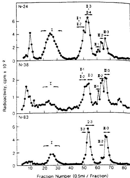
FIGURE 10: Ion-exchange HPLC of N-linked saccharides from N-24, N-38, and N-83 glycopeptides. N-linked saccharides obtained after Sephadex G-50 gel filtration (Figure 7) were applied to a column of TSK-DEAE 2SW equilibrated with 25 mM potassium phosphate buffer, pH 5.0. After being washed with the same buffer for 10 min, the column was eluted with a linear gradient from the same buffer to 400 mM potassium phosphate buffer, pH 5.0. The fractions were indicated by the same numbers as described previously (Sasaki et al., 1987). No carbohydrate was detected in other fractions. (Top) N-24 saccharides; (middle) N-38 saccharides; (bottom) N-83 saccharides.
