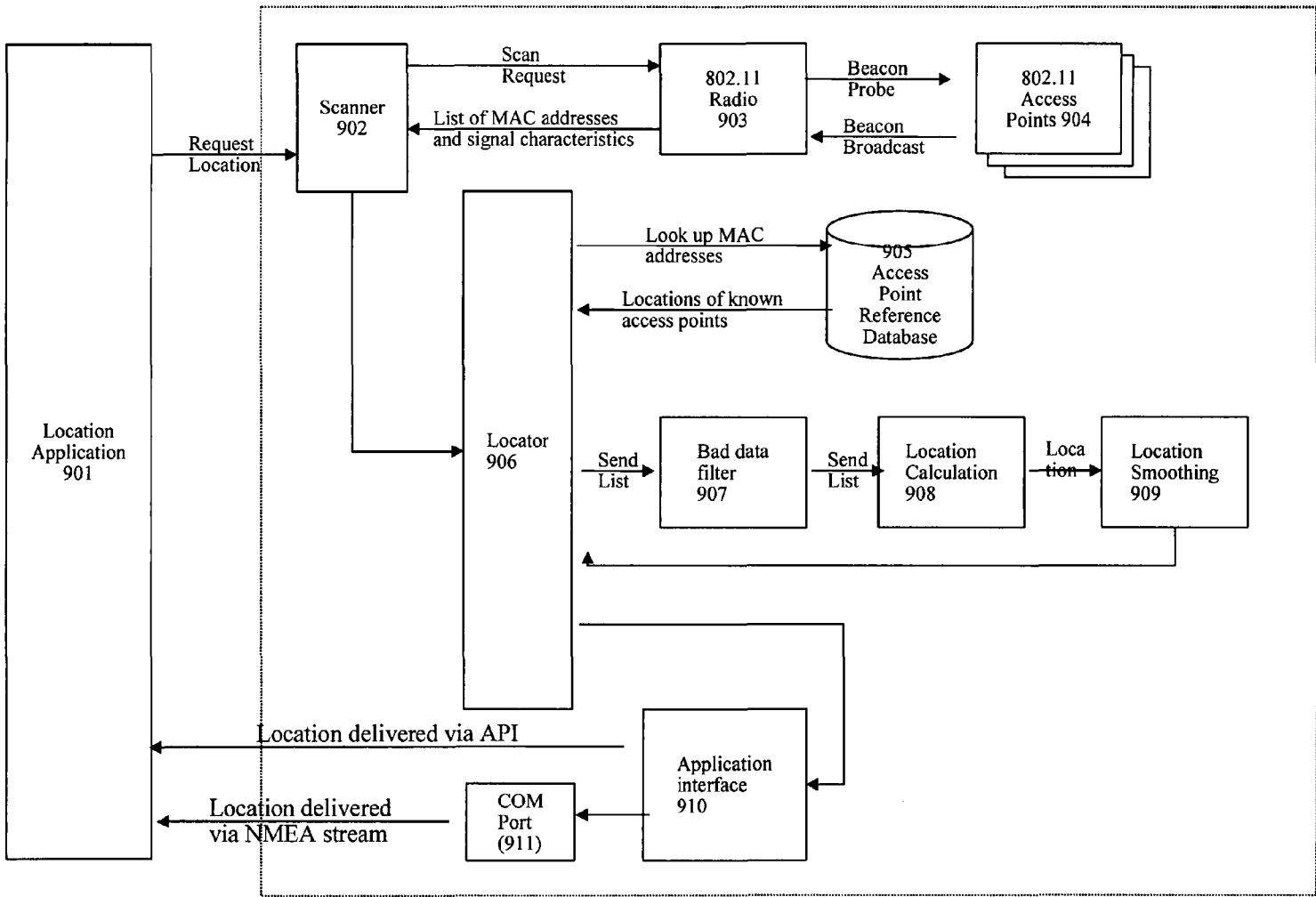
Figure 9: Positioning Software
