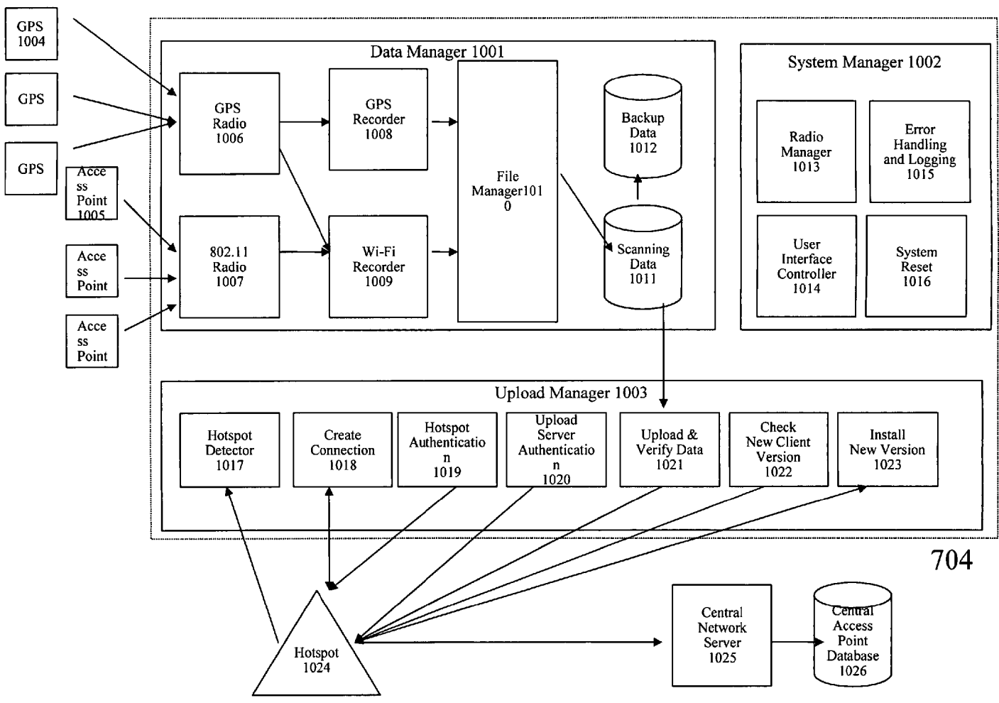
Figure 10: Scanning Client
