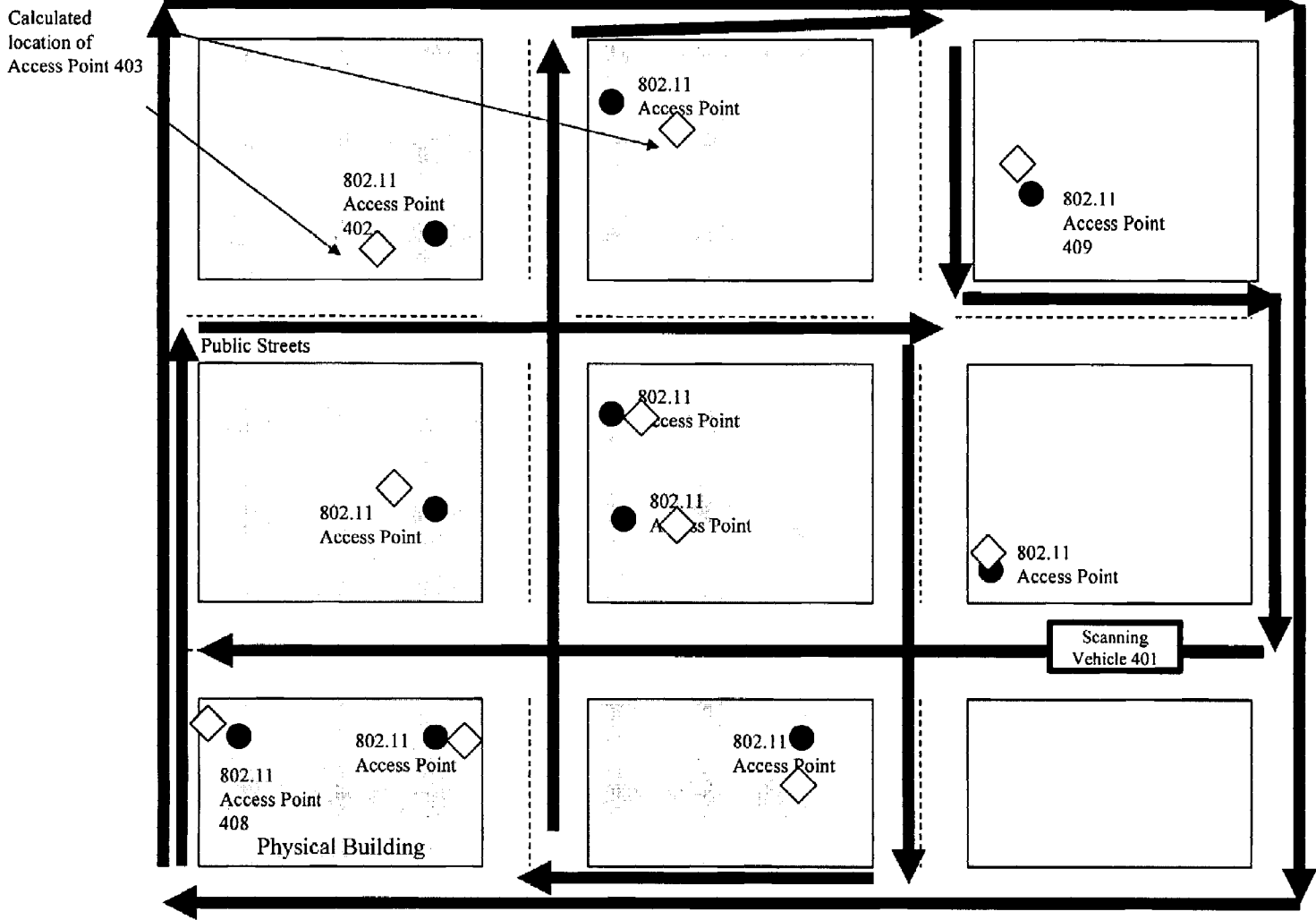
Figure 4: Chinese Postman routing
