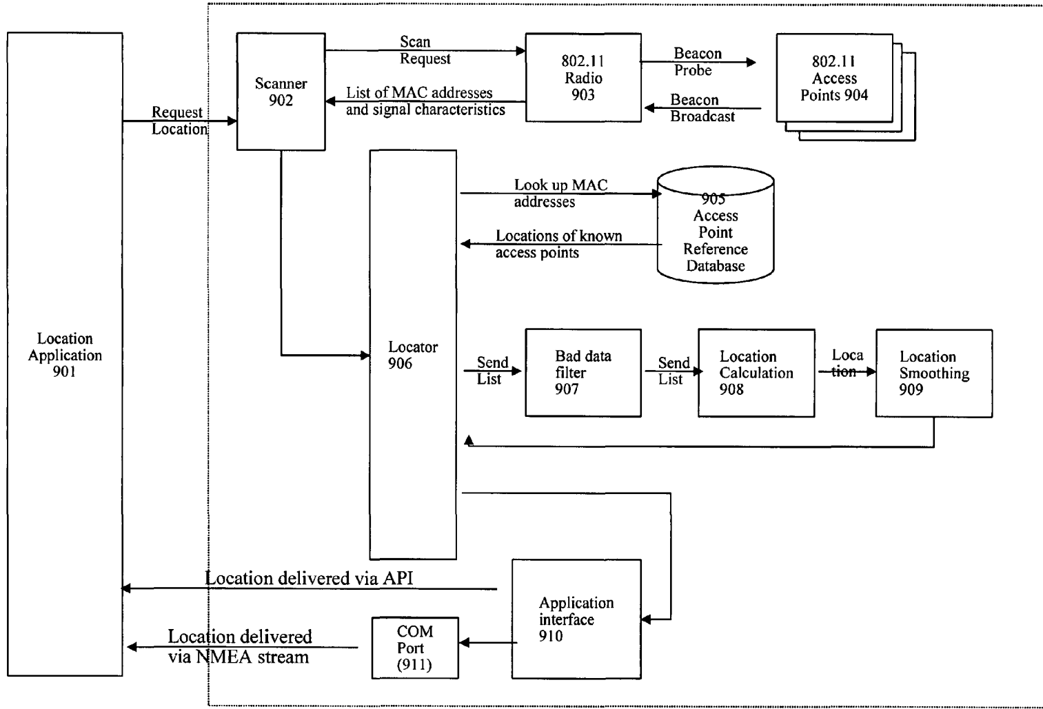
Figure 9: Positioning Software
