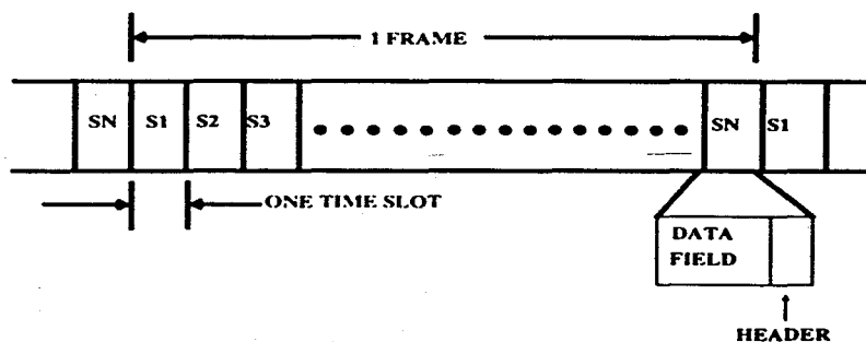
Figure 1.8. A hypothetical packet-interleaved transmission format. Here, a connection is identified either by a specifically numbered time slot reserved in each frame or by a connection identification number contained in the packet header.
