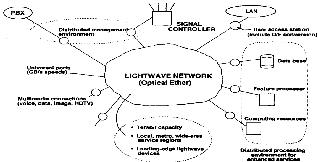
Figure 1.5. A distributed telecommunication network based on the notion of the "optical ether."
