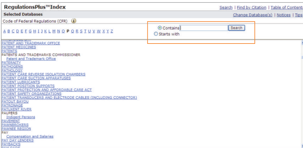
Figure 1. RegulationsPlus Index
