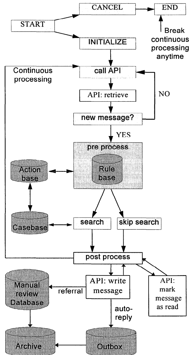
Figure 3. EZ Reader Internal Processing Flow
