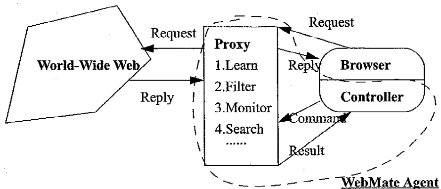
Figure 1: System Architecture
