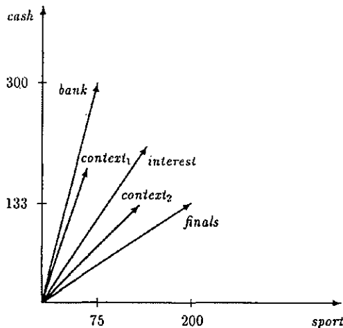
Figure 2: A vector model for context.
