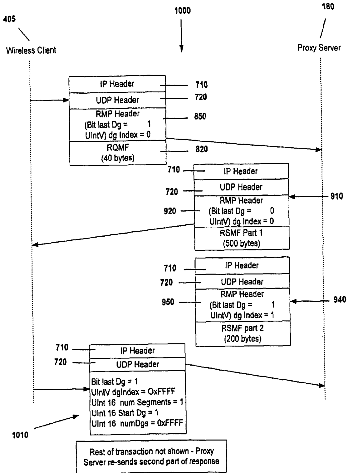
Figure 10- Exchange of Messages Including a Re-transmit Sequence
